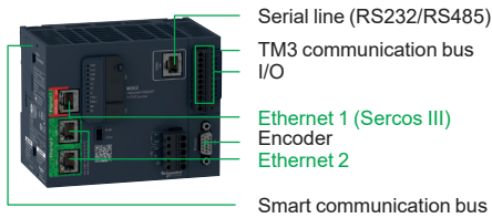
Modicon M262 motion controller
