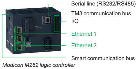
Modicon M262 logic controller
