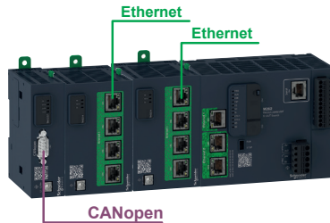
Modicon M262 logic controller with 3 Smart communication modules: 2x TMSES4 and 1x TMSCO1 (TMSCO1: always the last module on the left): Maximum configuration with CANopen
