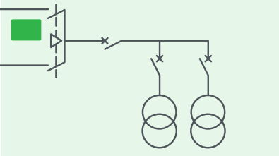
MV / LV consumer substation double feeder
